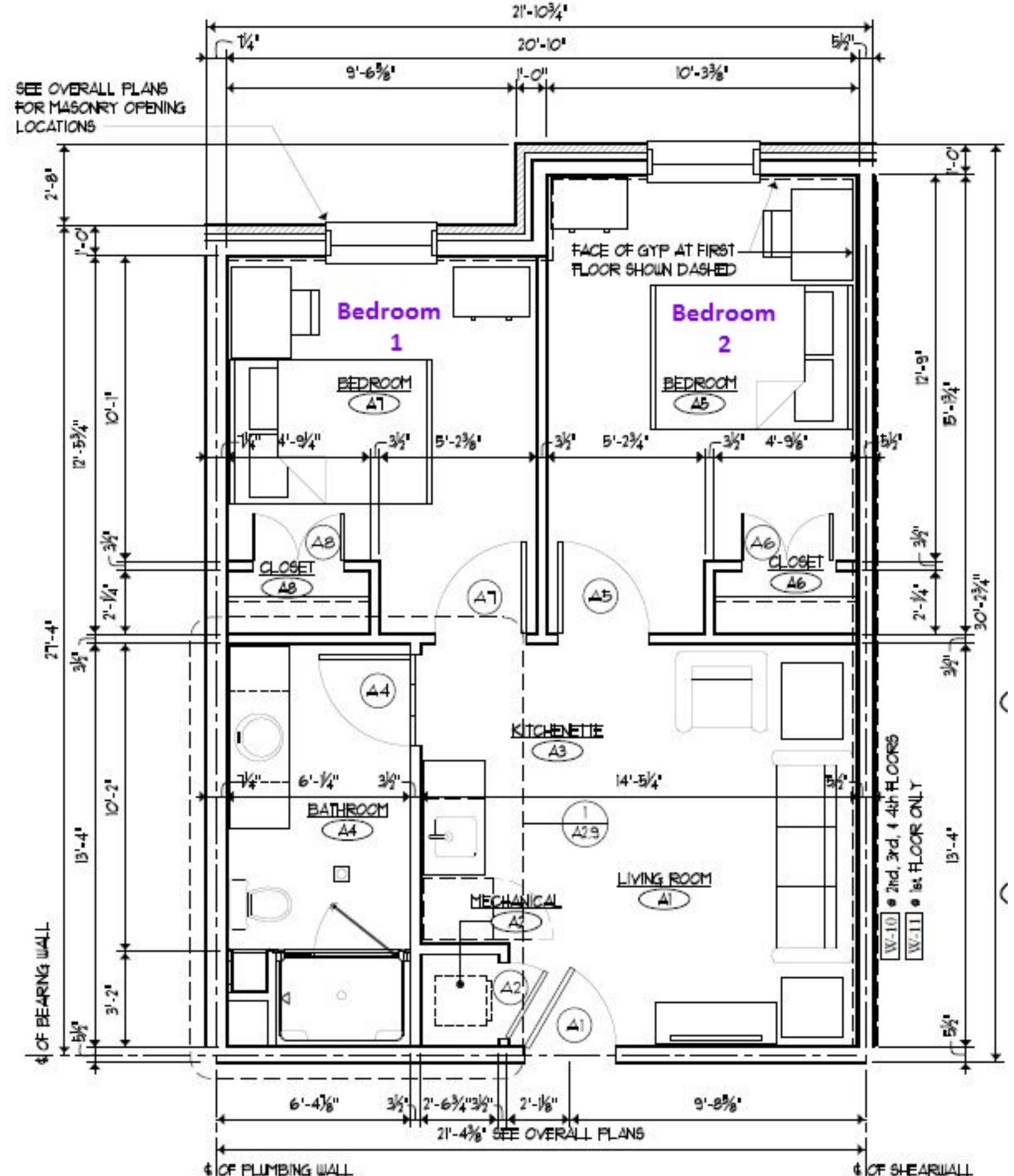
1 SUITE 'A' PLAN A2.6 1/4" = 1'-0"
