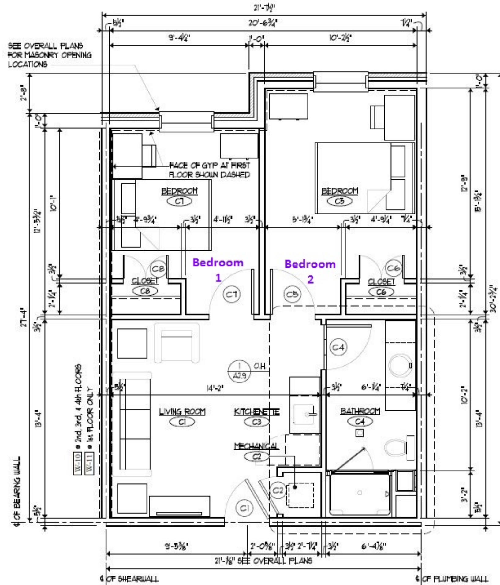
3 SUITE 'C' PLAN A2.6 1/4" = 1'-0"
