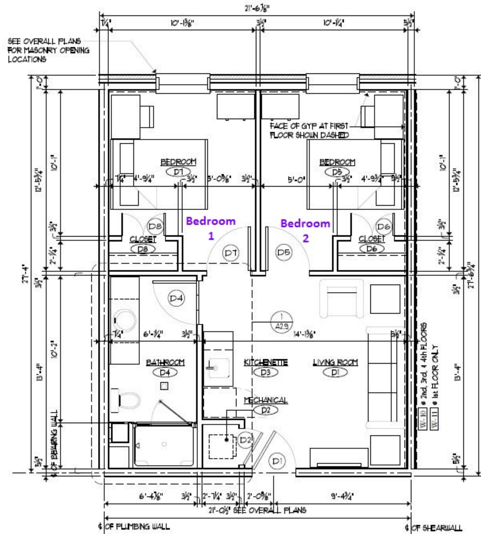
4 SUITE 'D' PLAN A2.6 1/4" = 1'-0"
