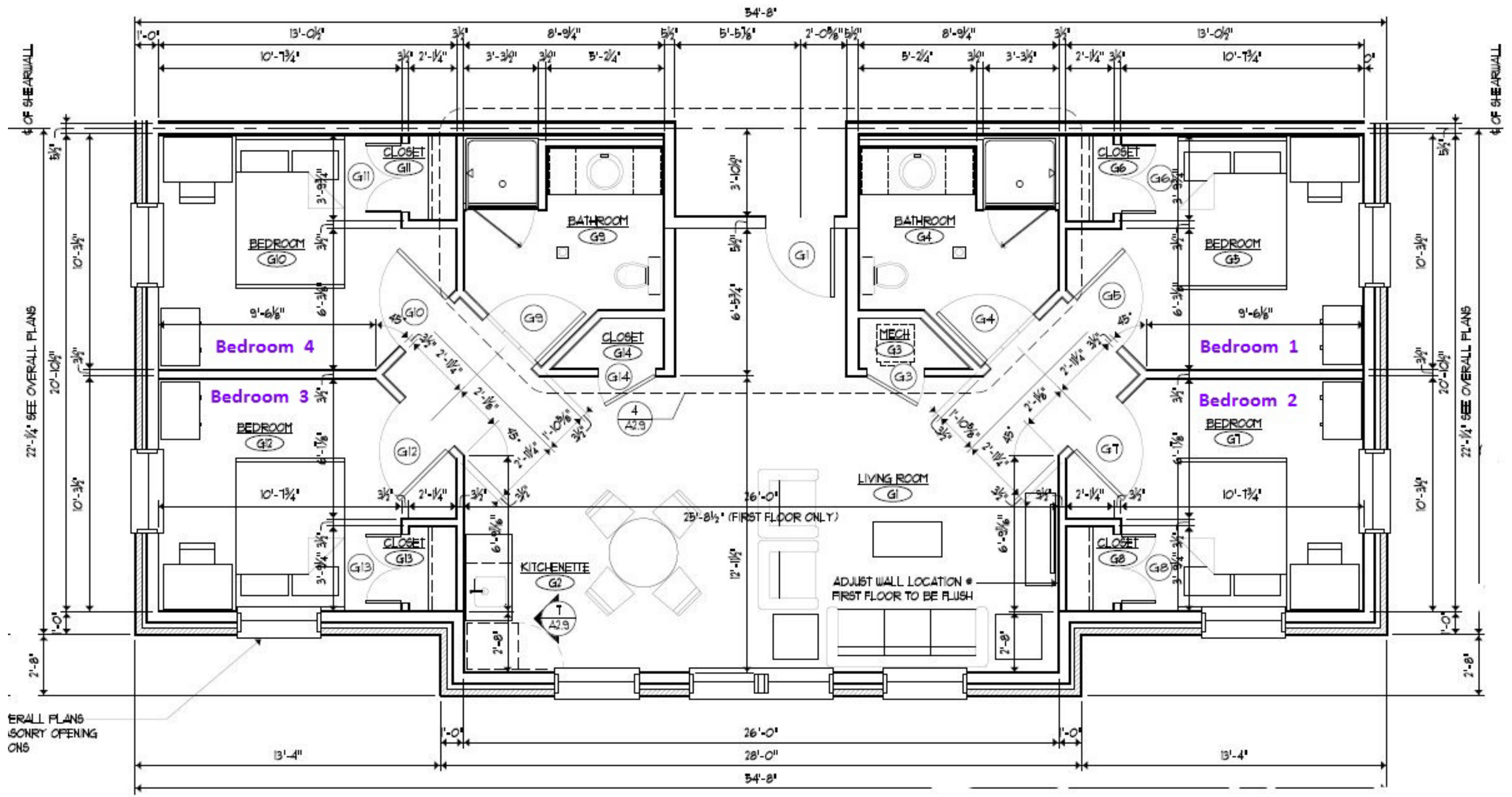
2 SUITE 'G' PLAN A2.7 1/4" = 1'-0"
