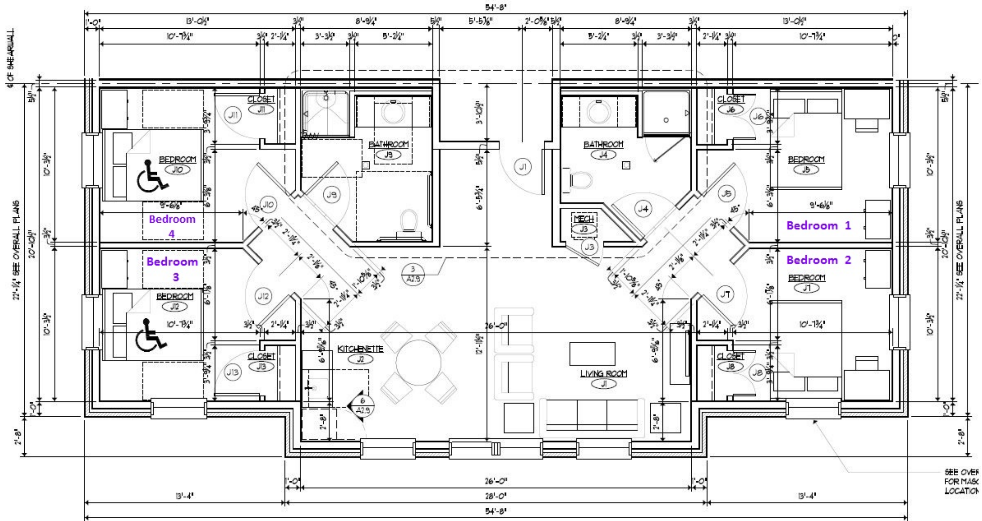
4 SUITE 'J' PLAN ACCESSIBLE A2.7 1/4" = 1'-0"
